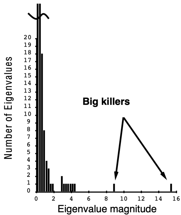
Fig. 20. Eigenvalue spectrum in a 4 layer shared weights network ( 256 \times 128 \times 64 \times 10 ) trained on 320 handwritten digits.
