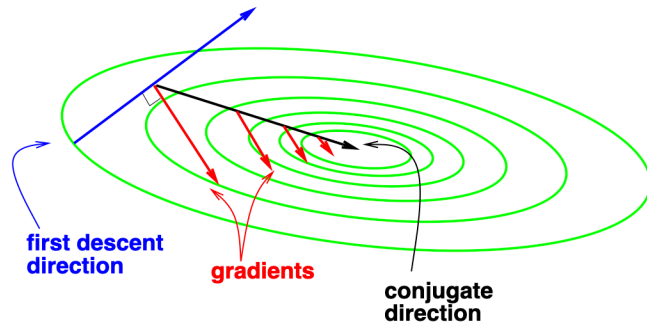
Fig. 16. Sketch of conjugate gradient directions in a 2D error surface.
