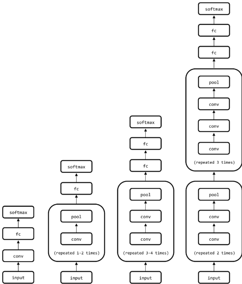
Figure 5-14. Various convolutional network architectures of various complexities. The architecture of VGGNet, a deep convolutional network built for ImageNet, is shown in the rightmost network.
