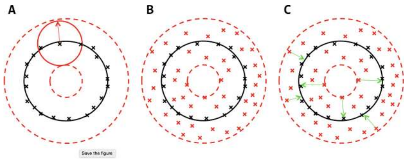
Figure 6-13. The denoising objective enables our model to learn the manifold (black circle) by learning to map corrupted data (red x 's) to uncorrupted data (black x 's) by minimizing the error (green arrows) between their representations
