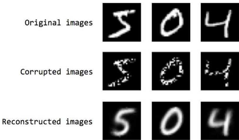
Figure 6-14. We apply a corruption operation to the dataset and train a denoising autoencoder to reconstruct the original, uncorrupted images
