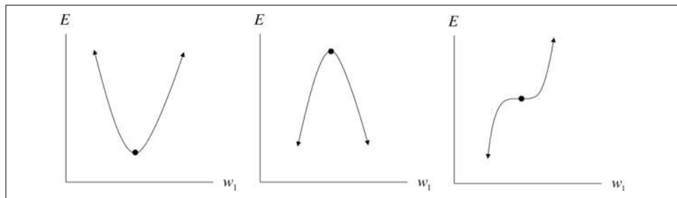
Figure 4-4. Analyzing a critical point along a single dimension
