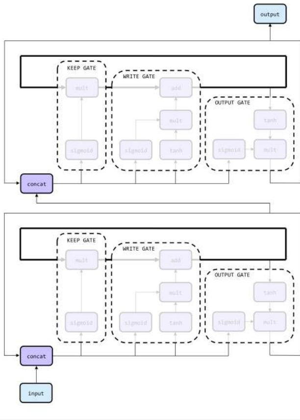
Figure 7-22. Composing LSTM units as one might stack recurrent layers in a neural network
