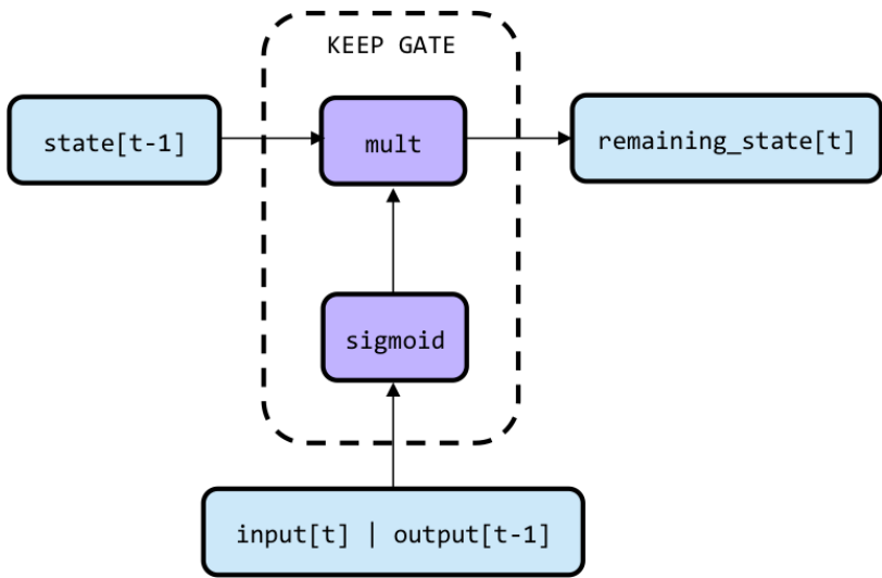
Figure 7-18. Architecture of the keep gate of an LSTM unit
