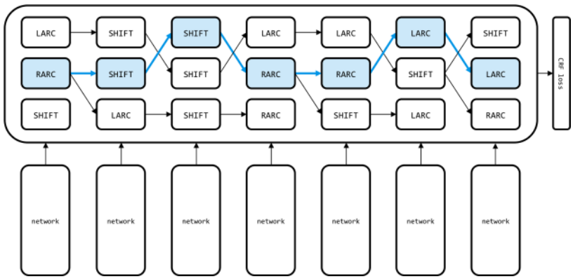
Figure 7-12. We can make global normalization in SyntaxNet tractable by coupling training and beam search
