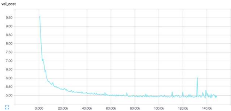
Figure 6-7. The cost incurred on the training set (logged after each minibatch) and on the validation set (logged after each epoch)
