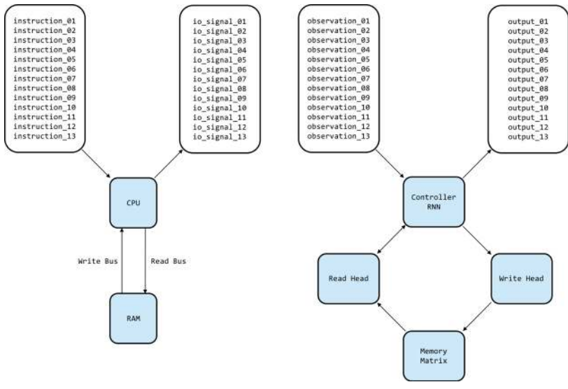
Figure 8-1. Comparing the architecture of a modern day computer which is fed its program (left) to a Neural Turing Machine that learns its program (right). This example has a single read head and single write head, but an NTM can have several in practice.
