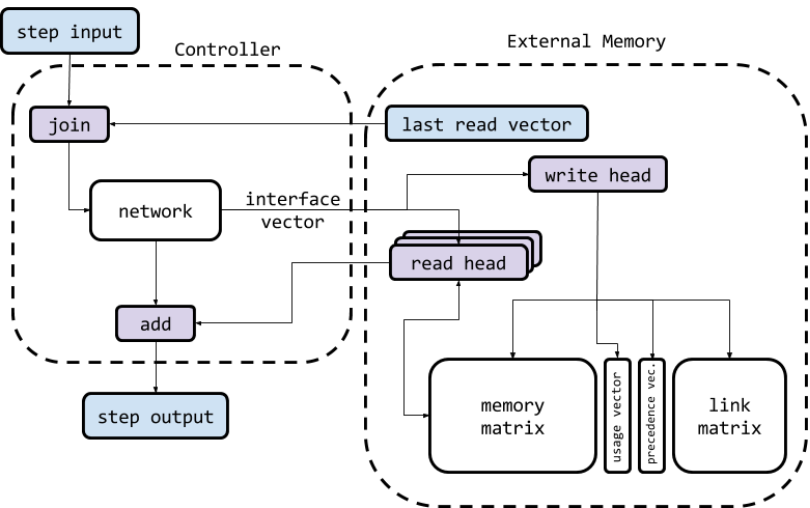
Figure 8-6. An overview of DNC's architecture and operation.
